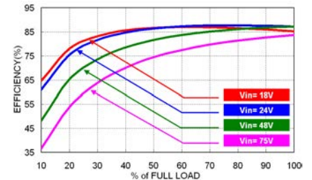
DFEC15-48S05W Efficiency vs. Output Load
