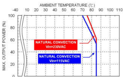
Derating Curve vs. Ambient Temperature TAD30USxxB xx=12/15/24/28/36/48/53 Connector Option : (Blank: JST)
