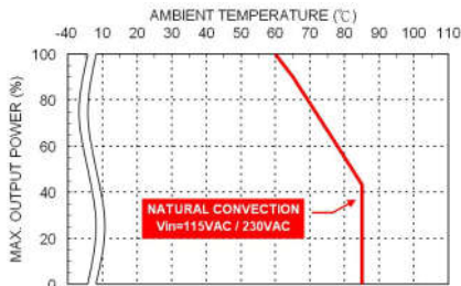
Derating Curve vs. Ambient Temperature TAD30USxxB xx=3P3/05/7P5/09/121/151/18 Connector Option : (Blank: JST)
